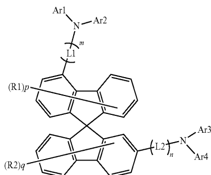
[Chemical Formula 1]
